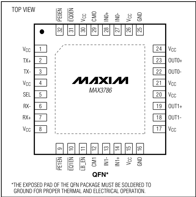
Pin Configuration
